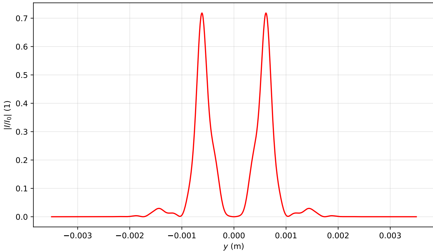
Intensity profile I(x=0, y, z=1.194)/I_0 , P_{in}=7.0P_{cr} , artificial time
